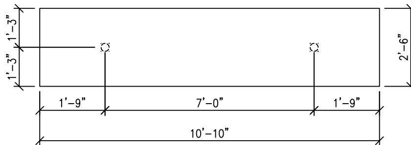
PLAN VIEW
