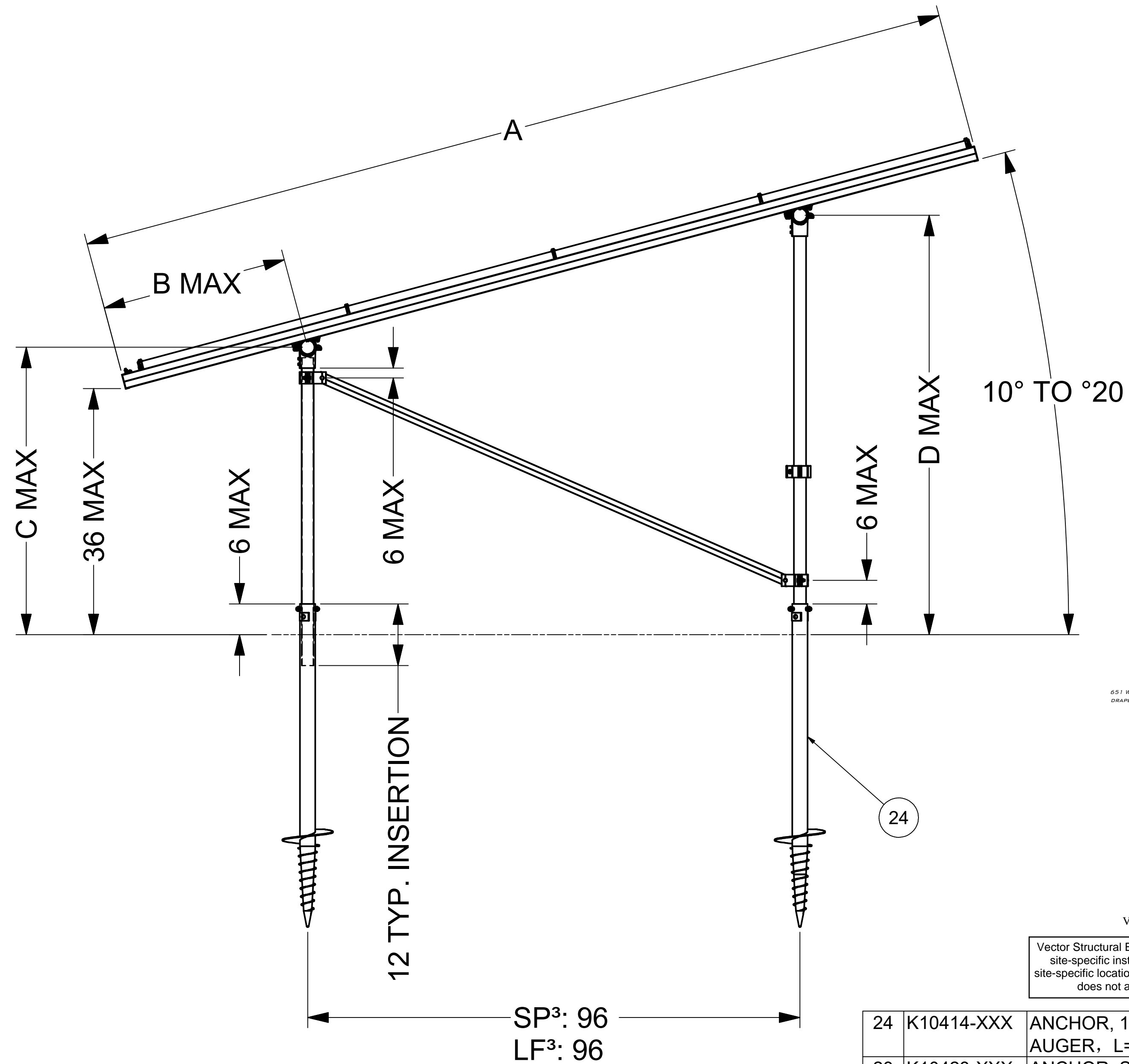
AUGER GROUND MOUNT (AGM) 4
