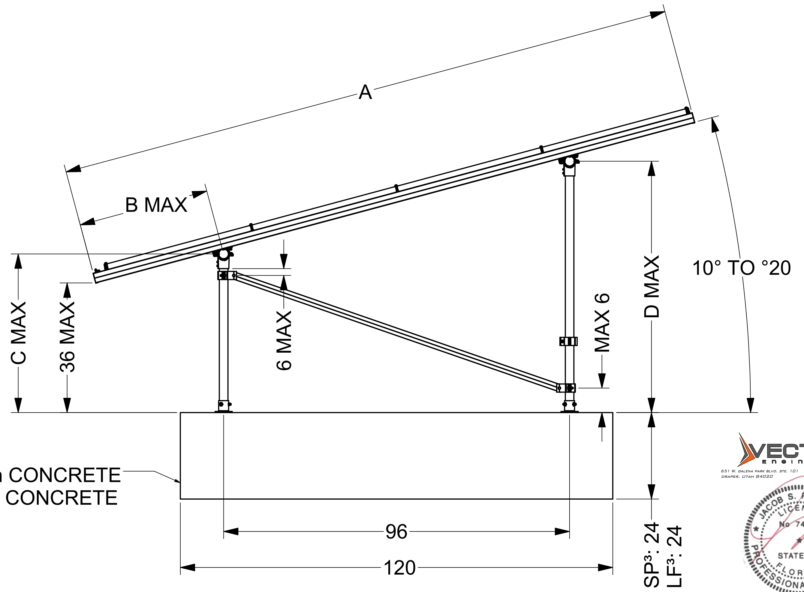
BALLAST GROUND MOUNT (BGM) 5
