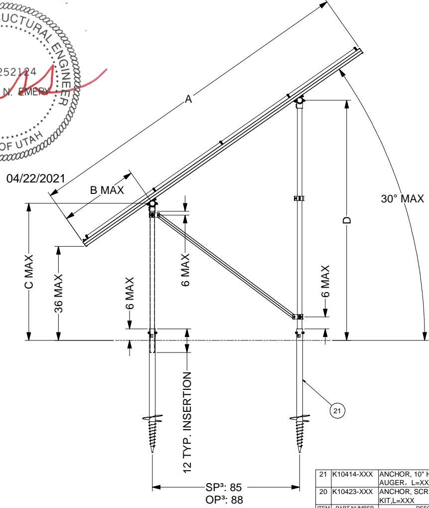
AUGER GROUND MOUNT (AGM)
