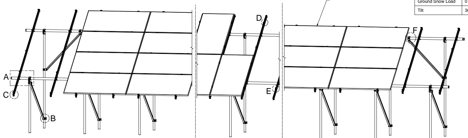
4L 4-IN-LANDSCAPE 2P 2-IN-PROTRAIT 3L 3-IN-LANDSCAPE STANDARD PANEL (SP) ONLY
