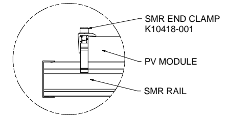
DETAIL G
