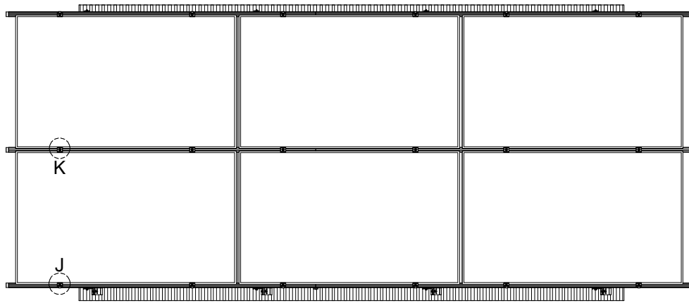
PLAN VIEW, SMR SYSTEM CORRUGATED METAL ROOF MOUNT, SHARED RAIL, LANDSCAPE MODULE
