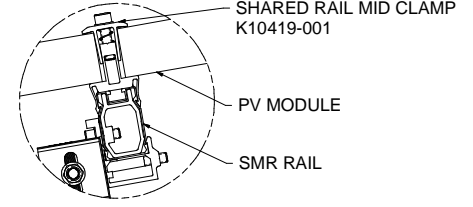
DETAIL M
