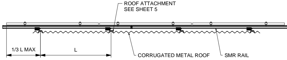
FRONT VIEW, SMR SYSTEM CORRUGATED METAL ROOF MOUNT, SHARED RAIL, LANDSCAPE MODULE
