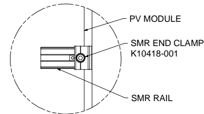
DETAIL E
