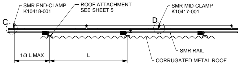
FRONT VIEW
