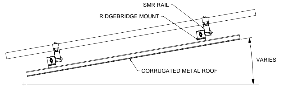
SIDE VIEW
