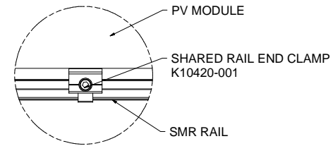
DETAIL J
