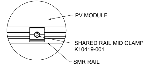
DETAIL K
