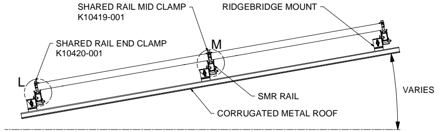
SIDE VIEW, SMR SYSTEM CORRUGATED METAL ROOF MOUNT, SHARED RAIL, LANDSCAPE MODULE
