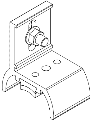
3/4 Pitch Height RidgeBridge Mount (no lag bolt) K10211-002
