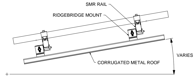
SIDE VIEW SMR SYSTEM CORRUGATED METAL ROOF MOUNT, LANDSCAPE MODULE
