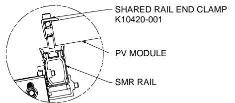
DETAIL L
