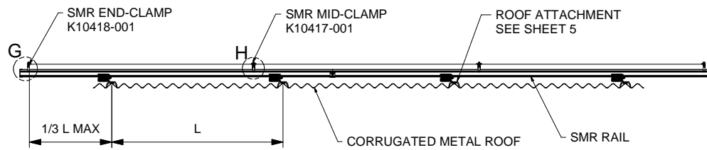
FRONT VIEW SMR SYSTEM CORRUGATED METAL ROOF MOUNT, LANDSCAPE MODULE
