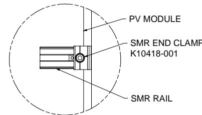
DETAIL E
