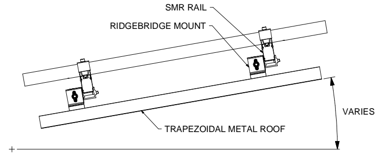
SIDE VIEW SMR SYSTEM TRAPEZOIDAL METAL ROOF MOUNT, LANDSCAPE MODULE
