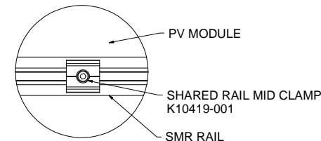
DETAIL K
