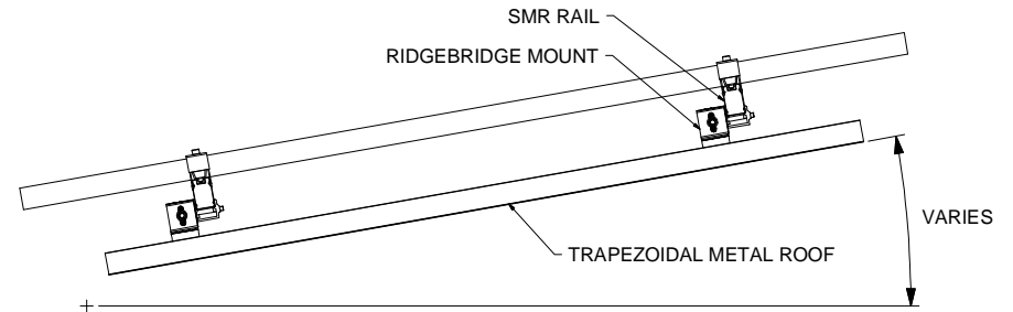
SIDE VIEW SMR SYSTEM TRAPEZOIDAL METAL MOUNT, PORTRAIT MODULE
