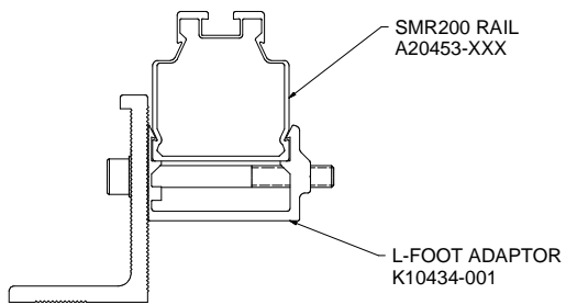
DETAIL, L-FOOT ADAPTOR, SMR200
