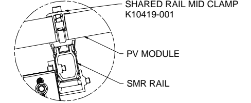
DETAIL M
