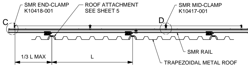
FRONT VIEW SMR SYSTEM TRAPEZOIDAL METAL ROOF MOUNT, PORTRAIT MODULE
