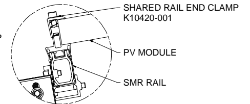
DETAIL L
