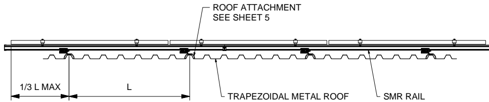
FRONT VIEW, SMR SYSTEM TRAPEZOIDAL METAL ROOF MOUNT, SHARED RAIL, LANDSCAPE MODULE
