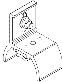
1 Pitch Height RidgeBridge Mount (no lag bolt) K10212-002
