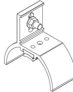
1-1/2 Pitch Height RidgeBridge Mount (no lag bolt) K10213-002
