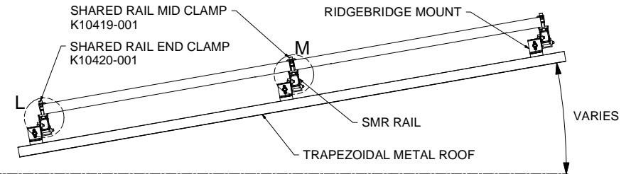
SIDE VIEW, SMR SYSTEM TRAPEZOIDAL METAL ROOF MOUNT, SHARED RAIL, LANDSCAPE MODULE
