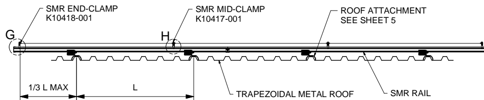
FRONT VIEW SMR SYSTEM TRAPEZOIDAL METAL ROOF MOUNT, LANDSCAPE MODULE
