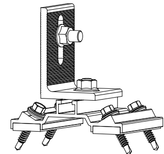
EZ Grip Metal Deck Mount (for 26ga SM) K50532-002
