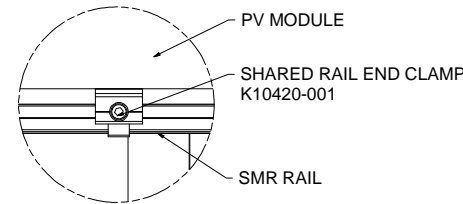
DETAIL J
