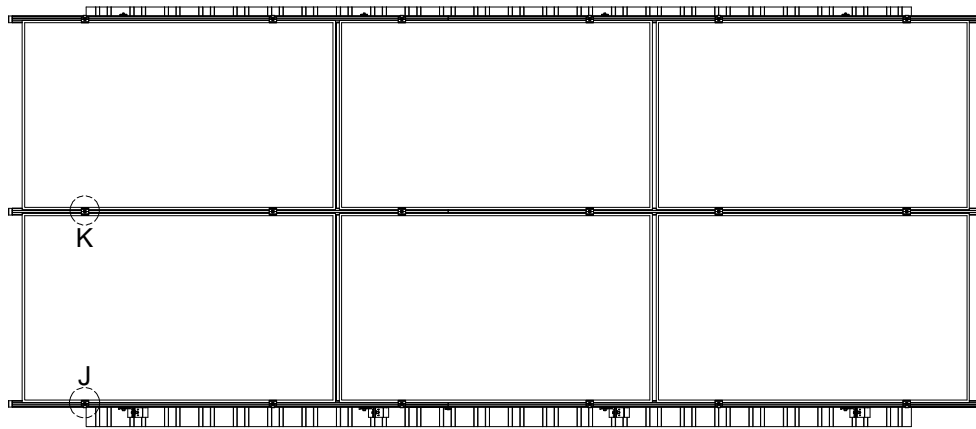
PLAN VIEW, SMR SYSTEM TRAPEZOIDAL METAL ROOF MOUNT, SHARED RAIL, LANDSCAPE MODULE
