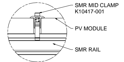
DETAIL D
