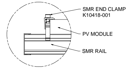
DETAIL G
