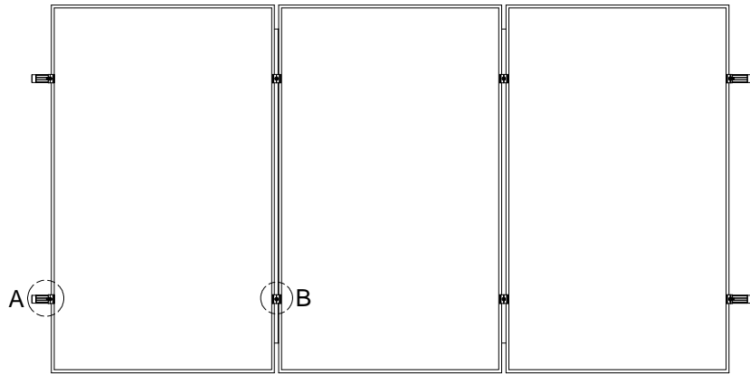
PLAN VIEW SMR SYSTEM TRAPEZOIDAL METAL ROOF MOUNT, PORTRAIT MODULE
