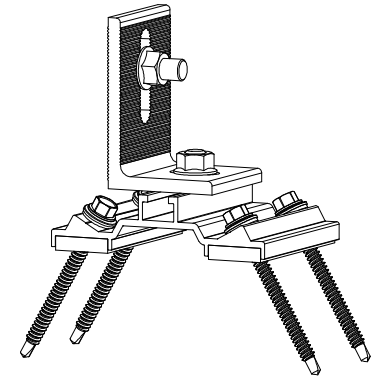
EZ Grip Metal Deck Mount K50532-001
