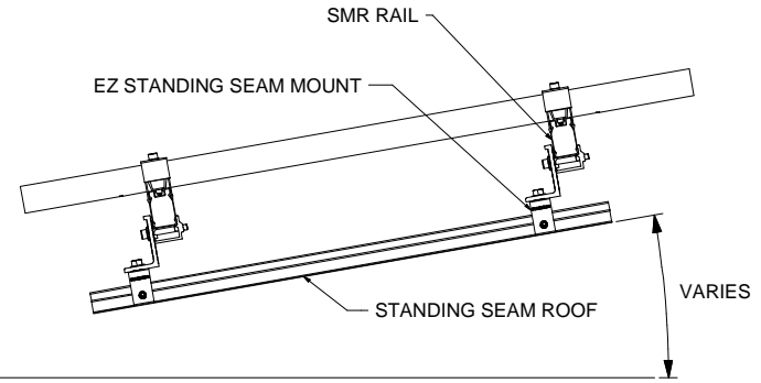
SIDE VIEW, SMR SYSTEM STANDING SEAM MOUNT, LANDSCAPE MODULE
