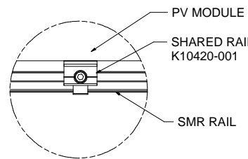
DETAIL J
