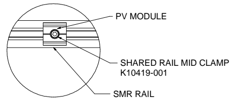
DETAIL K
