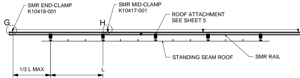
FRONT VIEW, SMR SYSTEM STANDING SEAM ROOF MOUNT, LANDSCAPE MODULE
