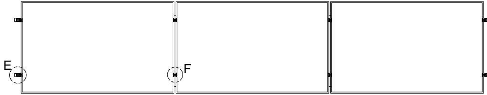
PLAN VIEW, SMR SYSTEM STANDING SEAM ROOF MOUNT, LANDSCAPE MODULE
