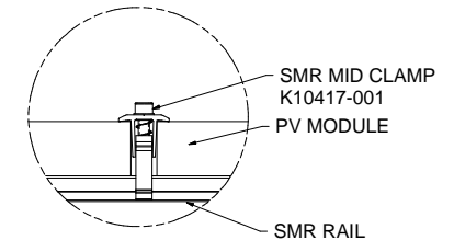
DETAIL H
