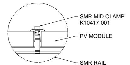
DETAIL D
