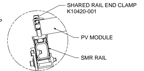
DETAIL L
