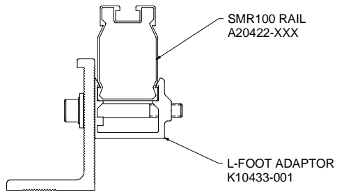
DETAIL, L-FOOT ADAPTOR, SMR100
