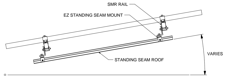
SIDE VIEW, SMR SYSTEM STANDING SEAM MOUNT, PORTRAIT MODULE
