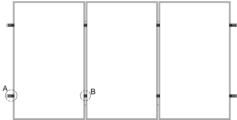
PLAN VIEW, SMR SYSTEM STANDING SEAM ROOF MOUNT, PORTRAIT MODULE
