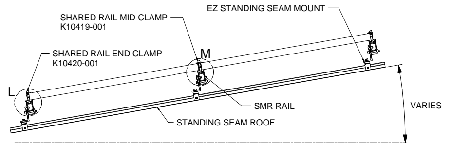
SIDE VIEW, SMR SYSTEM SHARED RAIL, LANDSCAPE MODULE
