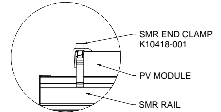
DETAIL G
