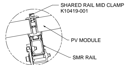
DETAIL M
