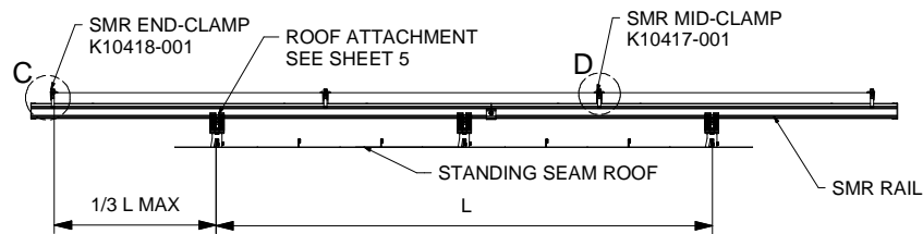
FRONT VIEW, SMR SYSTEM STANDING SEAM ROOF MOUNT, PORTRAIT MODULE
