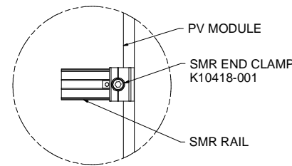
DETAIL E
