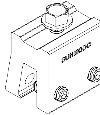
1" EZ STANDING SEAM CLAMP, STANDARD K50200-001
