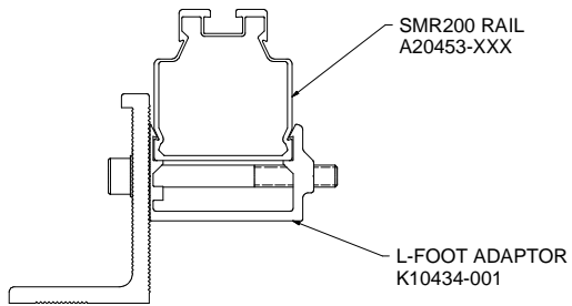
DETAIL, L-FOOT ADAPTOR, SMR200
