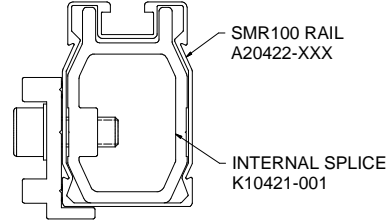
DETAIL, SPLICE, SMR100
