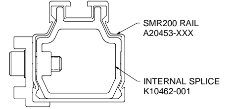
DETAIL, SPLICE, SMR200
