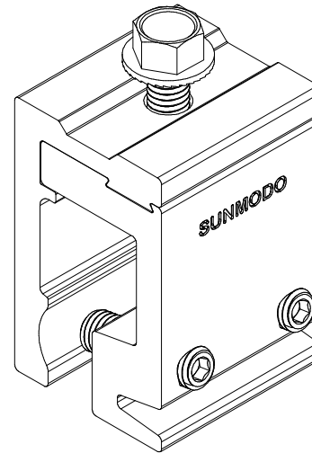
2" EZ STANDING SEAM CLAMP, STANDARD K50210-001
