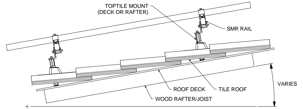
SIDE VIEW, SMR SYSTEM TILE ROOF MOUNT, PORTRAIT MODULE
