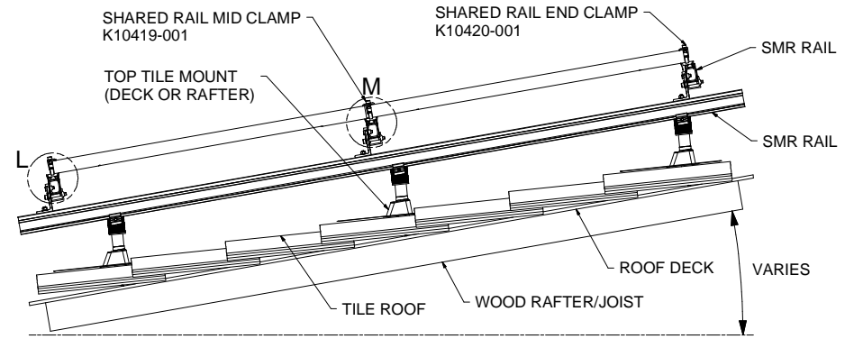
SIDE VIEW, SMR SYSTEM SHARED RAIL, LANDSCAPE MODULE
