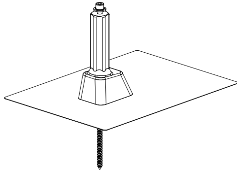
TOPTILE MOUNT K10466-XXX [RAFTER MOUNT]
