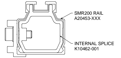
DETAIL, SPLICE, SMR200
