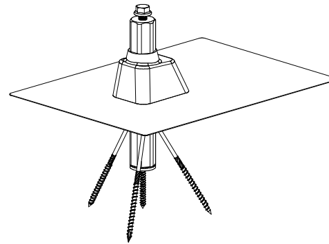
TOPTILE MOUNT K10461-XXX [DECK MOUNT]
