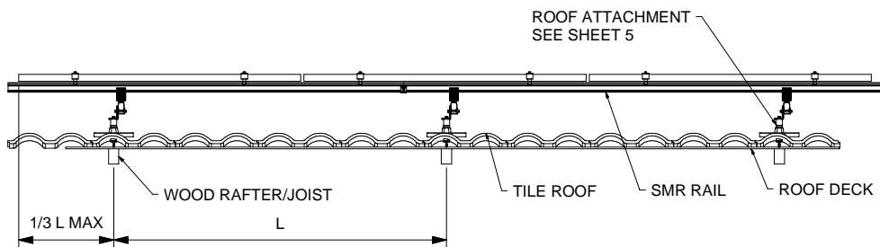
FRONT VIEW, SMR SYSTEM SHARED RAIL, LANDSCAPE MODULE
