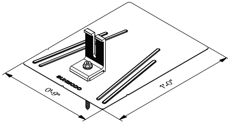
SOLOFLASH K50538-003 [RAFTER MOUNT]
