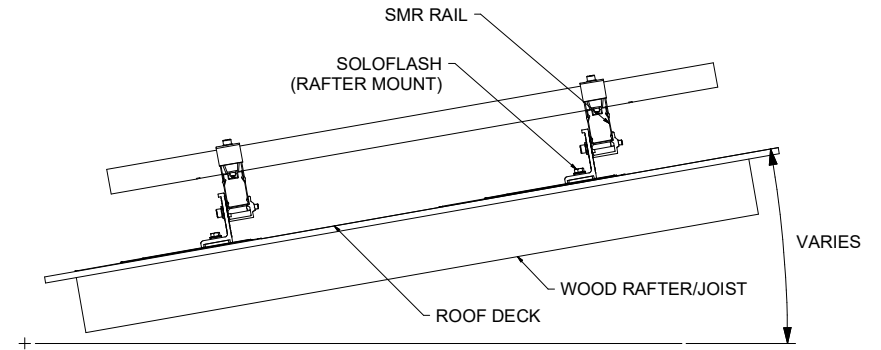
SIDE VIEW, SMR SYSTEM RAFTER MOUNT, LANDSCAPE MODULE
