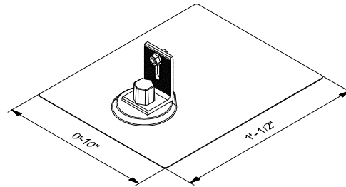
EZ ROOF MOUNT K10068-001 [RAFTER MOUNT]
