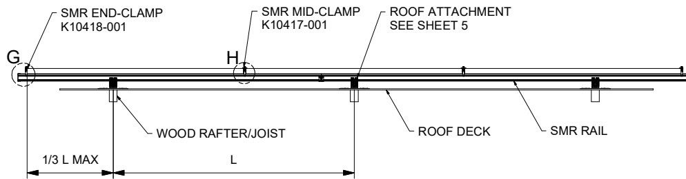
FRONT VIEW, SMR SYSTEM RAFTER MOUNT, LANDSCAPE MODULE
