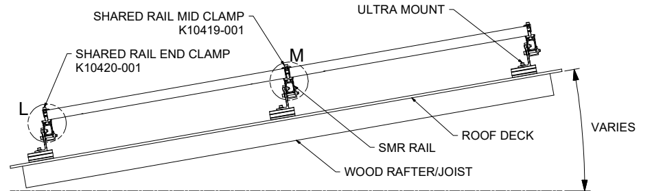
SIDE VIEW, SMR SYSTEM SHARED RAIL, LANDSCAPE MODULE
