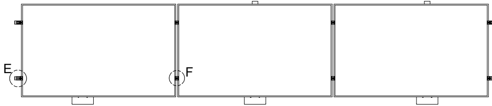
PLAN VIEW, SMR SYSTEM RAFTER MOUNT, LANDSCAPE MODULE
