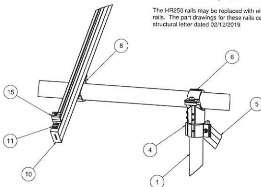
DETAIL E
